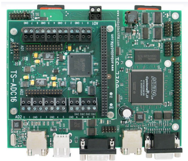
The TS-7300 computer with IO.
