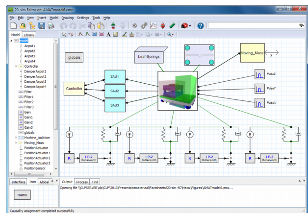
Model of the active vibration controller.
